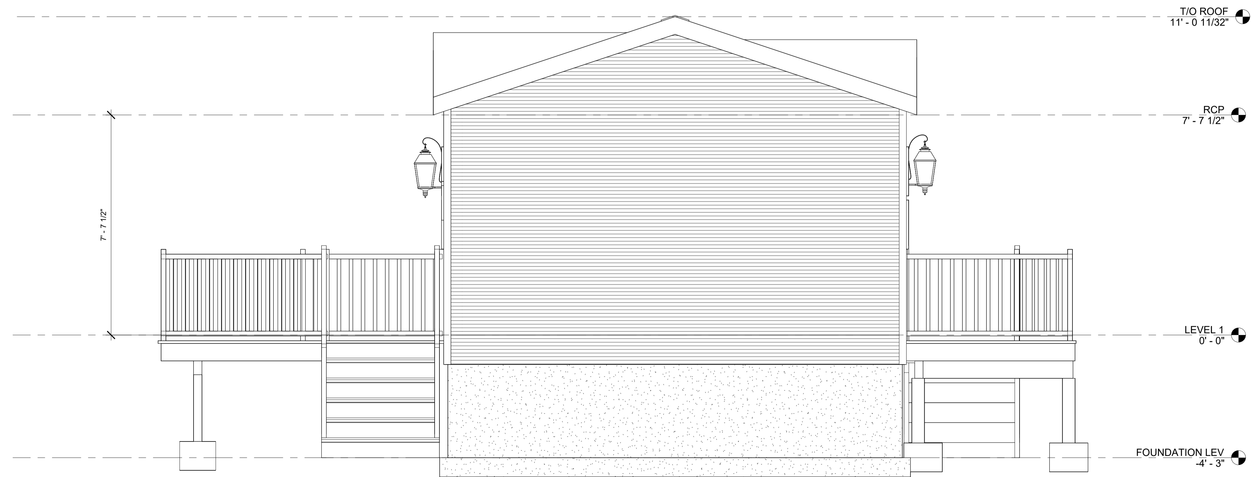
② RIGHT ELEVATION 1/2" = 1'-0"
