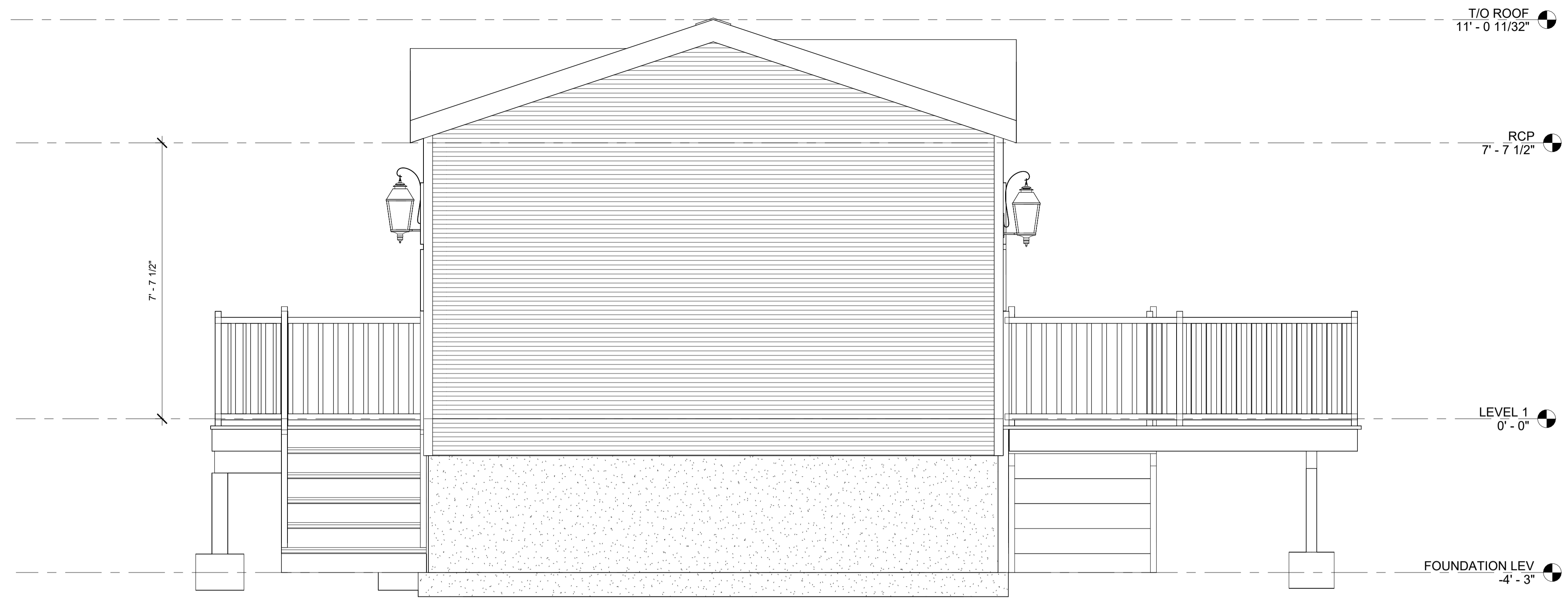
① LEFT ELEVATION 1/2" = 1'-0"
